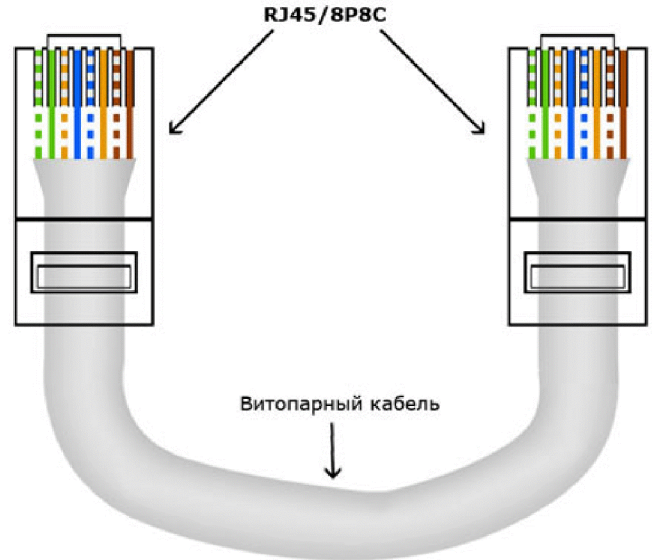
EIA/TIA-568A
