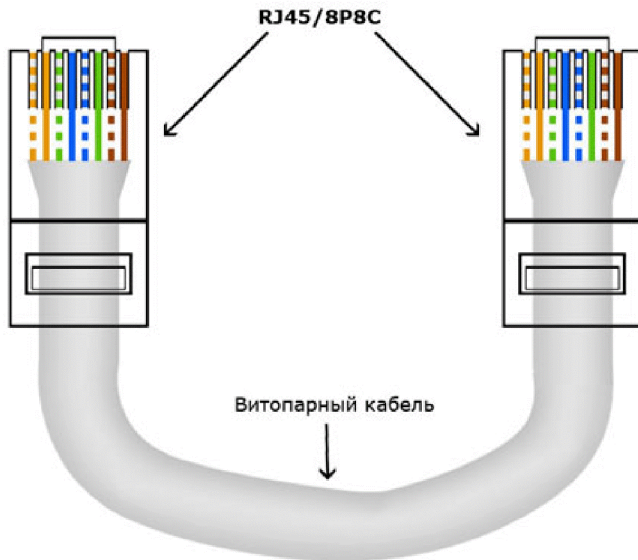
EIA/TIA-568B
